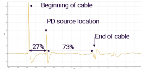
Figure 2 PD Waveform Analysis on HV Cable
